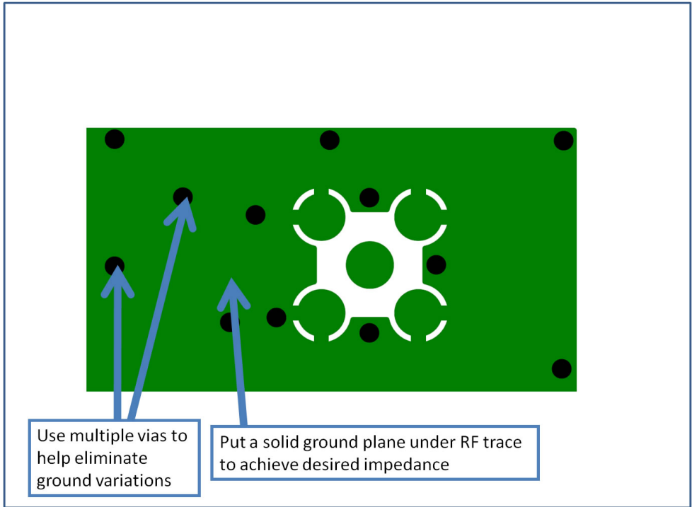
The following illustration shows PCB layer 2 of an example RF layout.
